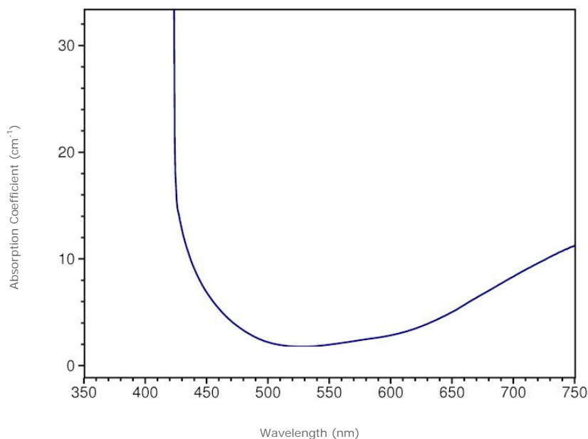
Visible Absorption | min. path length: 6.9 mm
