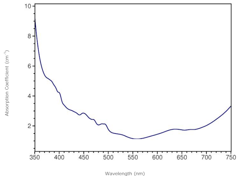
Visible Absorption | min. path length: 9.7 mm
