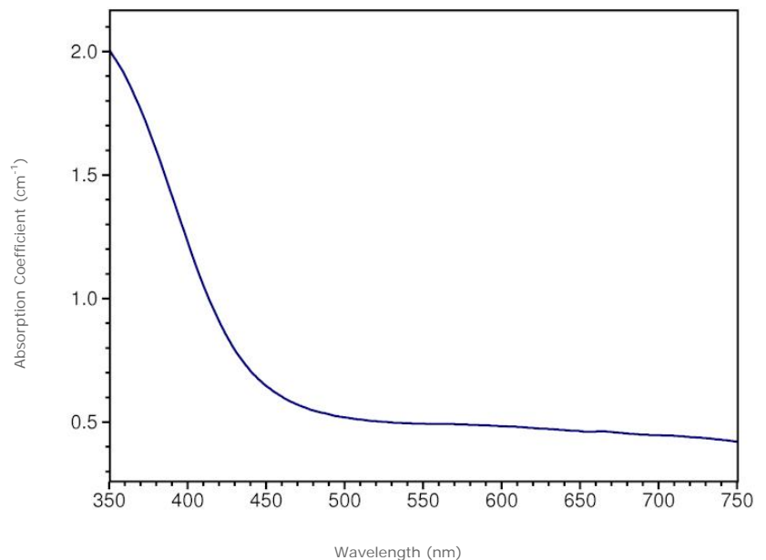
Visible Absorption | min. path length: 13.4 mm
