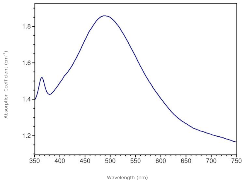
Visible Absorption | min. path length: 15.9 mm
