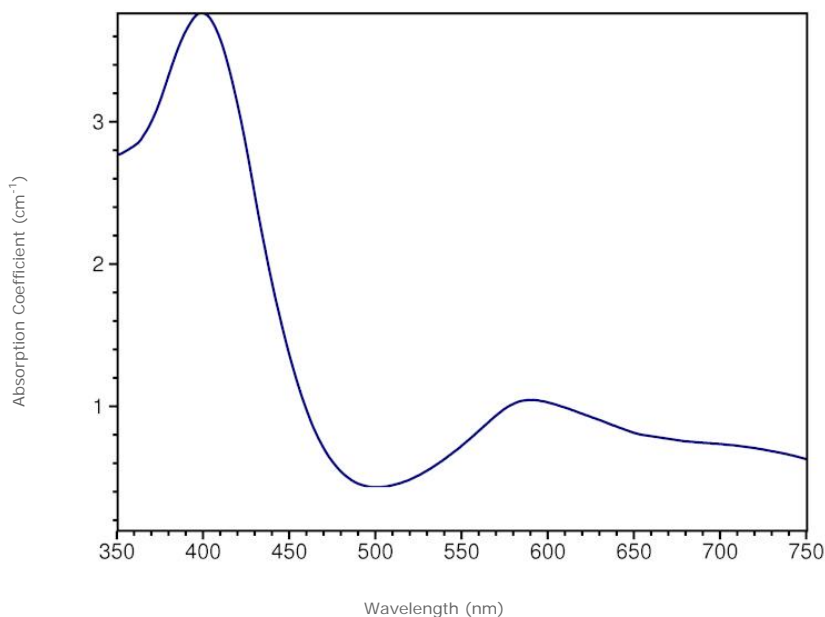
Visible Absorption | min. path length: 14.2 mm
