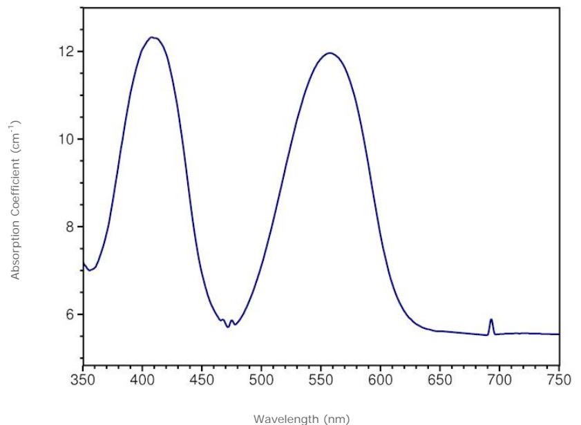
Visible Absorption | min. path length: 3.1 mm
